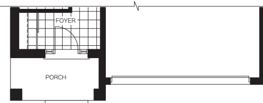
PARTIAL GROUND FLOOR ELEV. B
