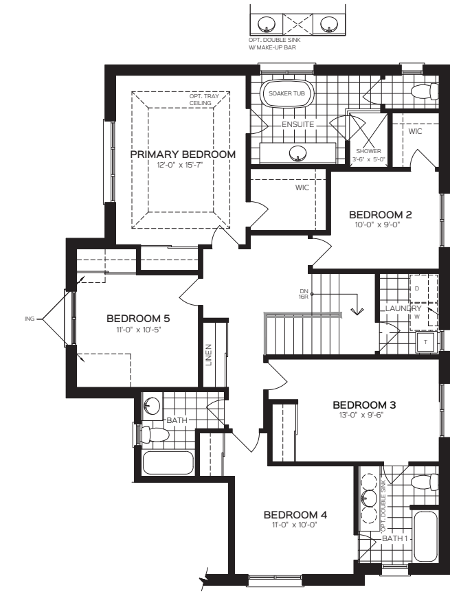
OPTIONAL SECOND FLOOR ELEV. B
