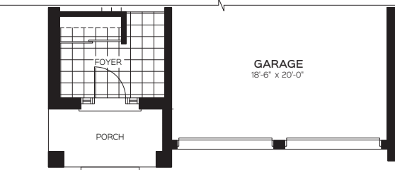
PARTIAL GROUND FLOOR ELEV. B
