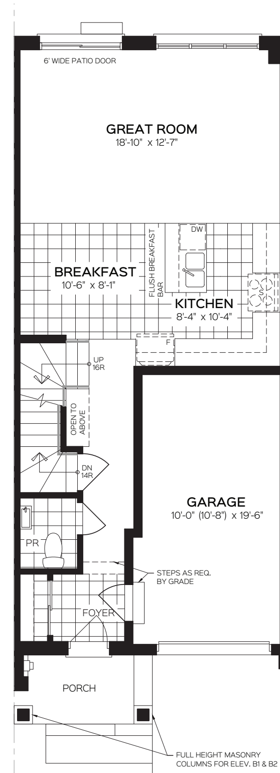
GROUND FLOOR ELEV. A1, A2, B1 & B2
